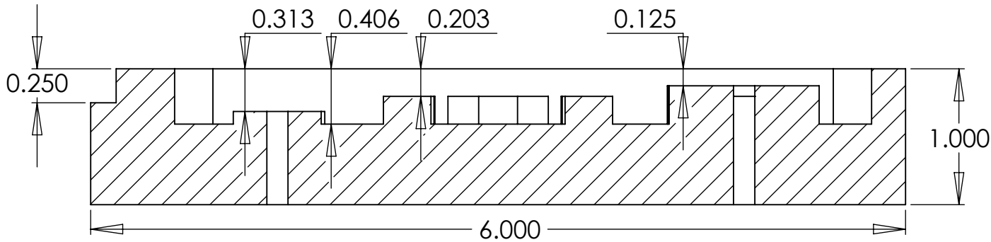
SECTION K-K SCALE 1 : 1
